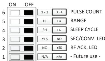
Factory Default Settings Outlined in BOLD Figure 7. DIP Switches
