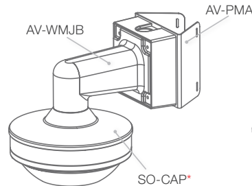
Wall Mount Configuration with Pole Mount Adapter
