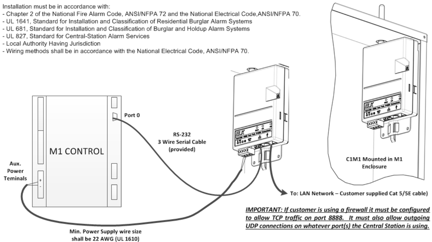
TYPICAL INSTALLATION LAYOUT
