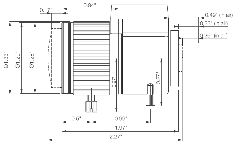
CLS2812D2.7-5mp
