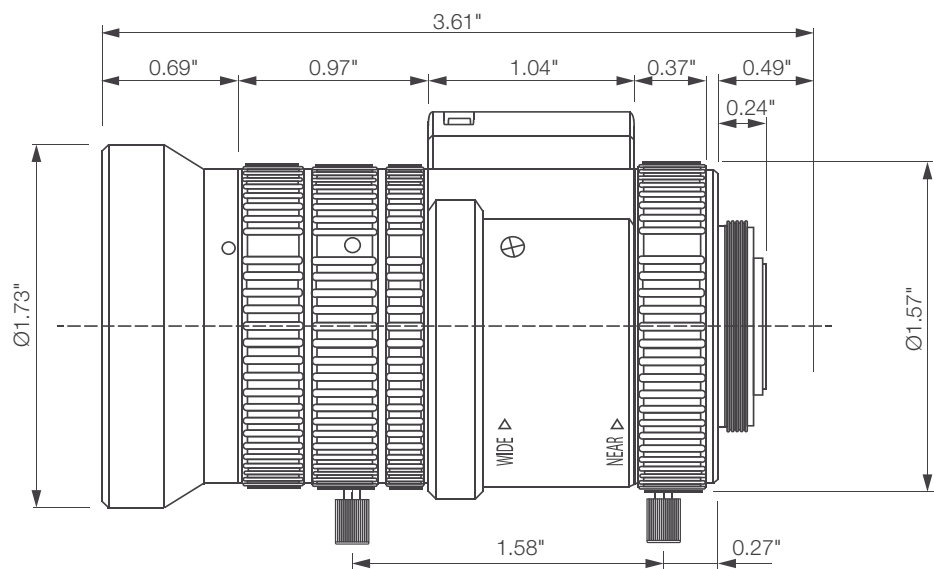
CLS5500D2.7-5mp
