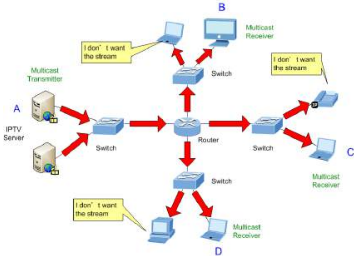
Figure 4-12-2 Multicast Flooding
