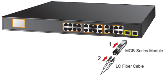
Figure 3-4: Plugging in the SFP Transceiver
