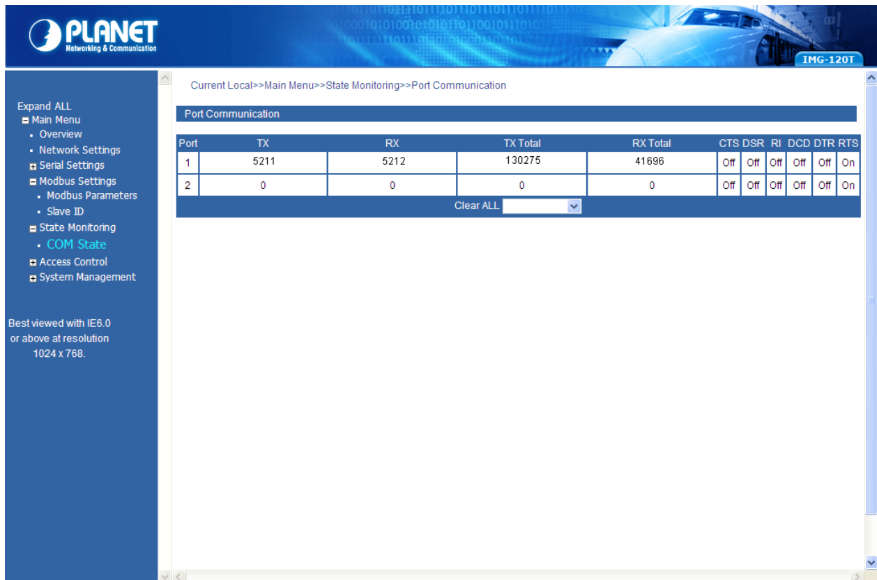
Figure 4-17: State Monitoring -- COM State Screen
