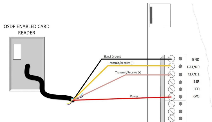
Figure 3.5: OSDP Wiring
