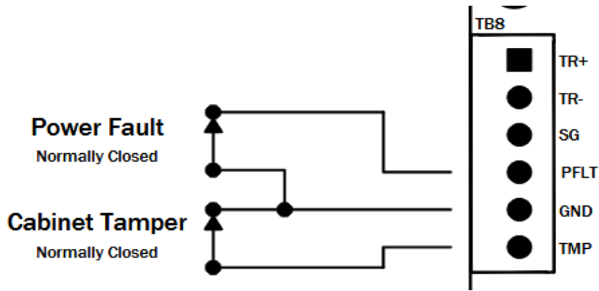
Figure 3.3: Cabinet Tamper & Power Fault Wiring
