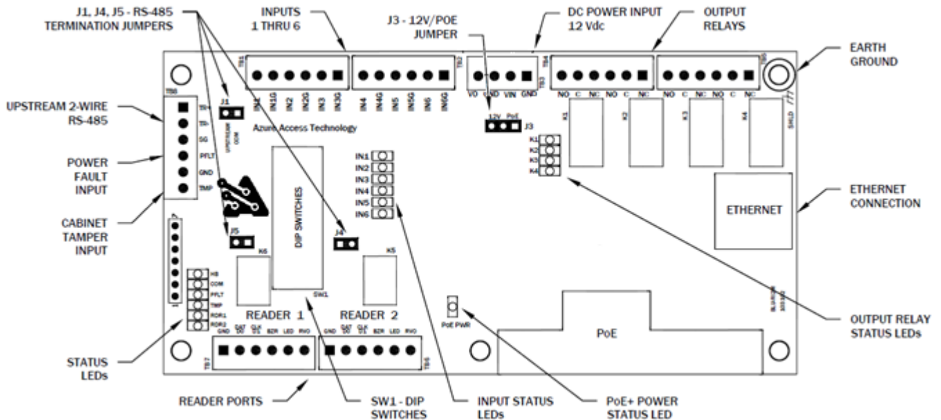
Figure 2.1: Board Diagram
