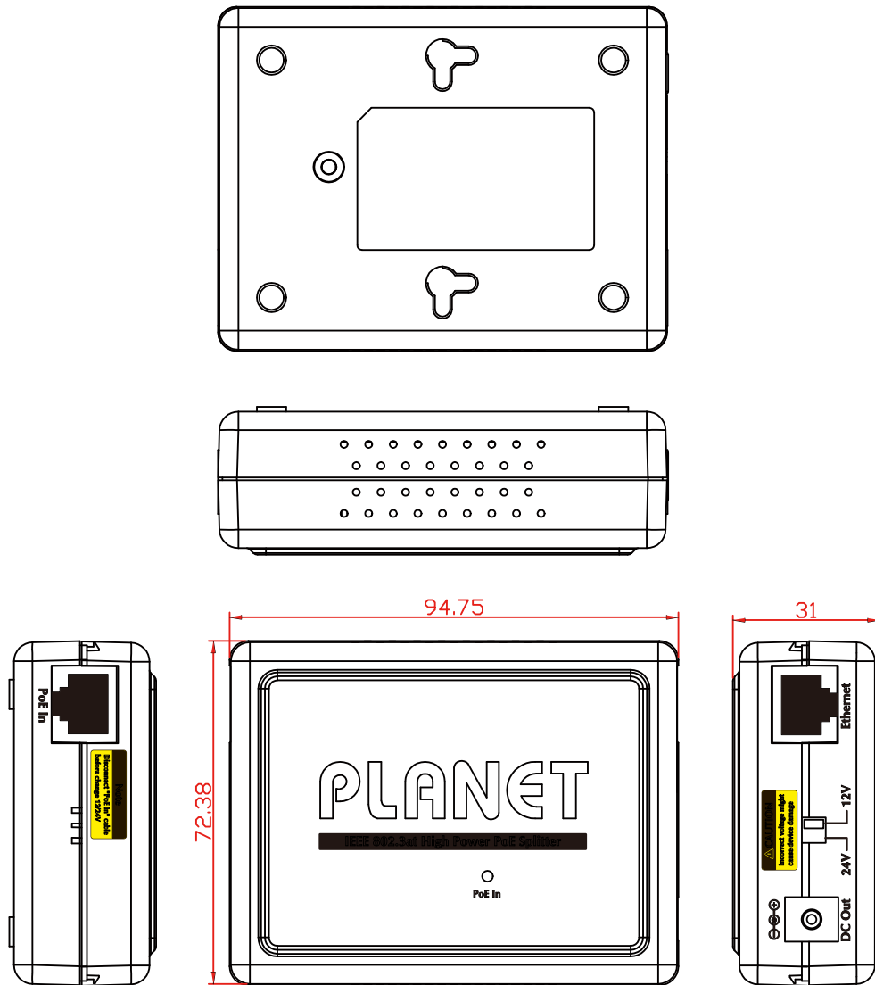
Dimension (unit = mm)
