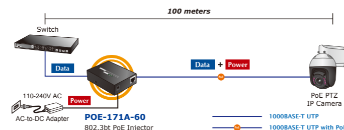
Figure 3: Architecture of Connected IEEE 802.3af/at/bt Devices
