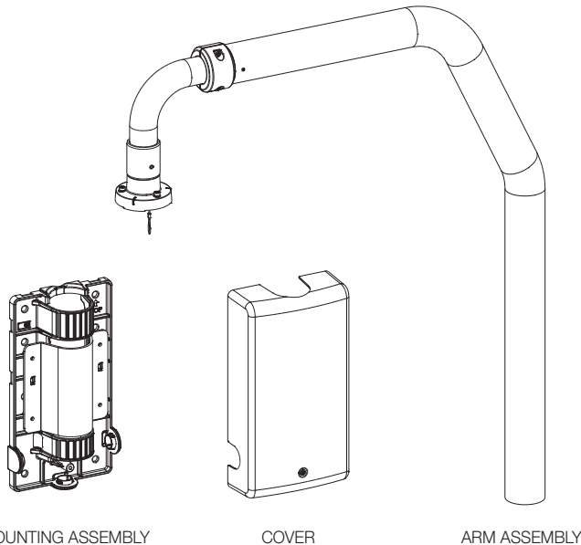
MOUNTING ASSEMBLY
