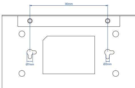
VC-234G Switch Bottom Side
