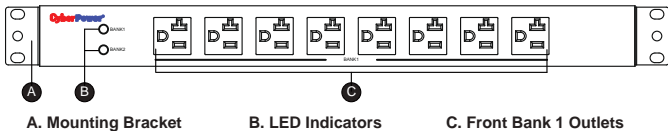
A. Mounting Bracket
