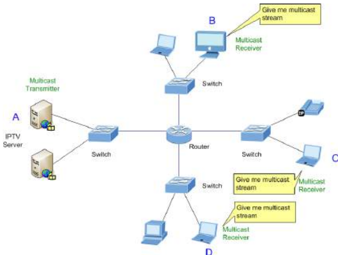
Figure 4-12-1 Multicast Service
