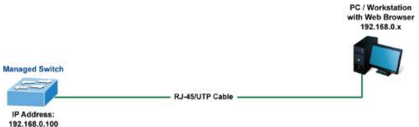
Figure 3-1 Web Management
