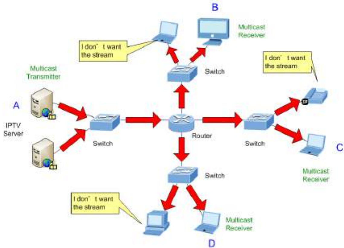
Figure 4-12-2 Multicast Flooding
