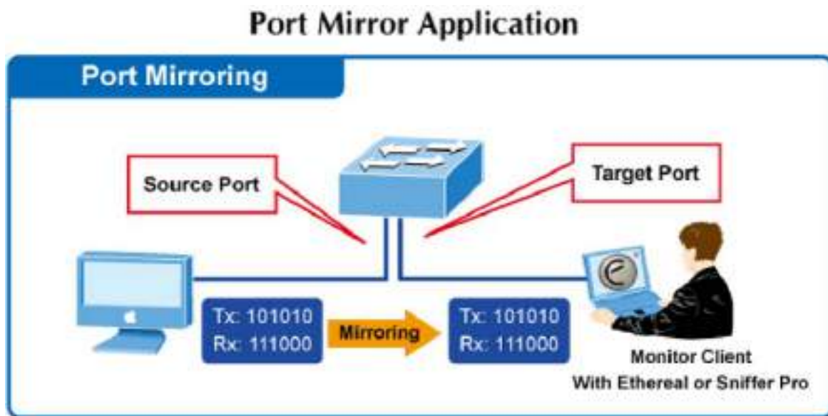
Figure 4-3-2 Port Mirror Application
