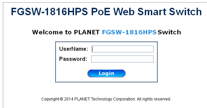
Figure 4-2 Login Screen
