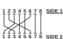
Figure A-1: Straight-Through and Crossover Cable
