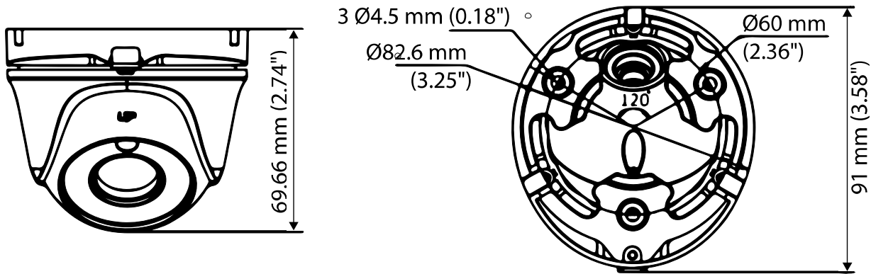
ECI-T12F2 Camera
