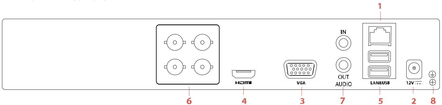
ERT-K2041 DVR Rear Panel
