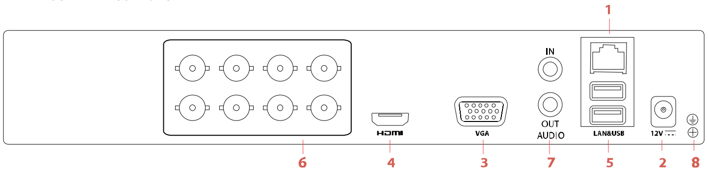
ERT-K2082 DVR Rear Panel
